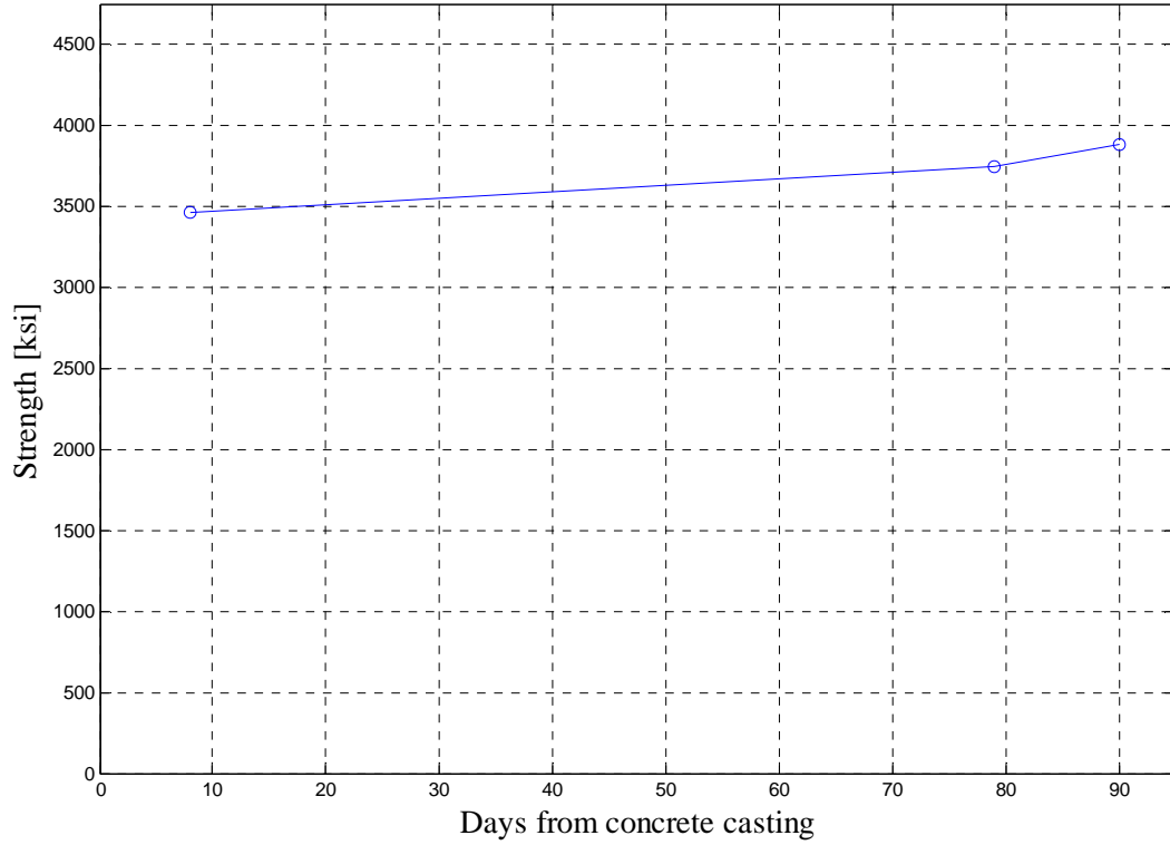
Figure A.2 E-MOD history for the column conventional concrete.
