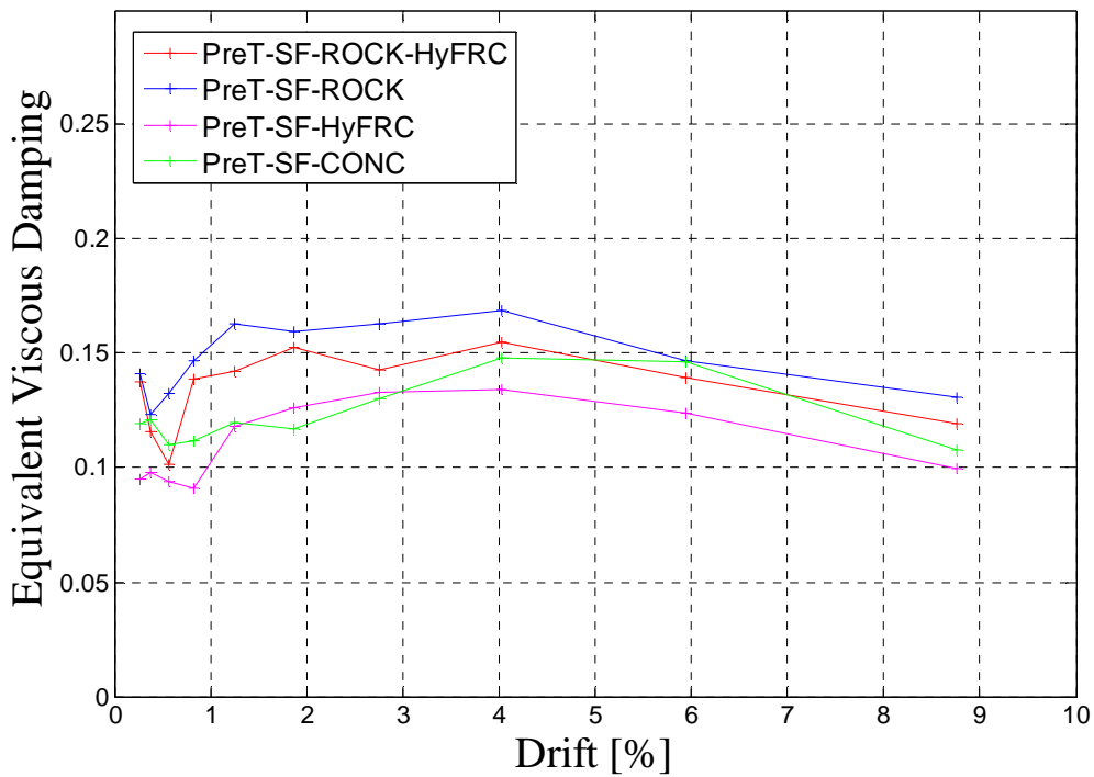
Figure 6.8 Equivalent viscous damping versus drift ratio.
