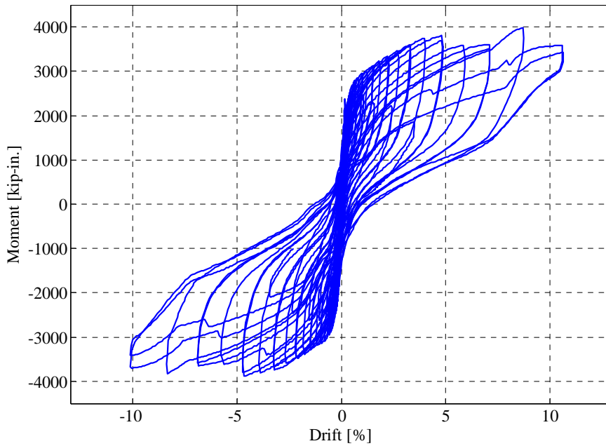
Figure 5.5 Uncorrected moment-drift plot for Specimen PreT-SF-ROCK.
